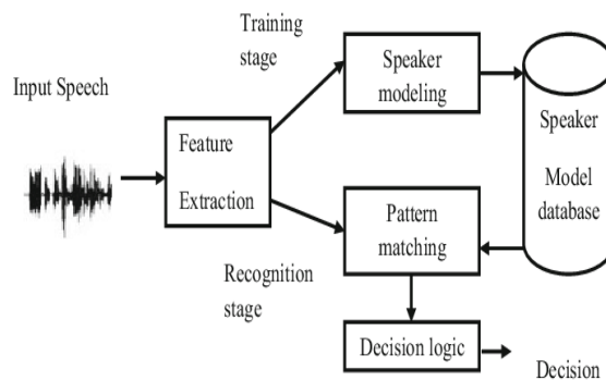
Fig 5. Existing voice recognition system for android
