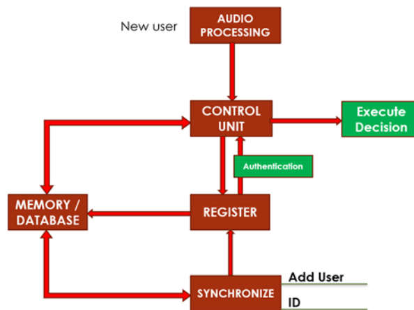
Fig 5. Proposed Voice recognition block diagram
